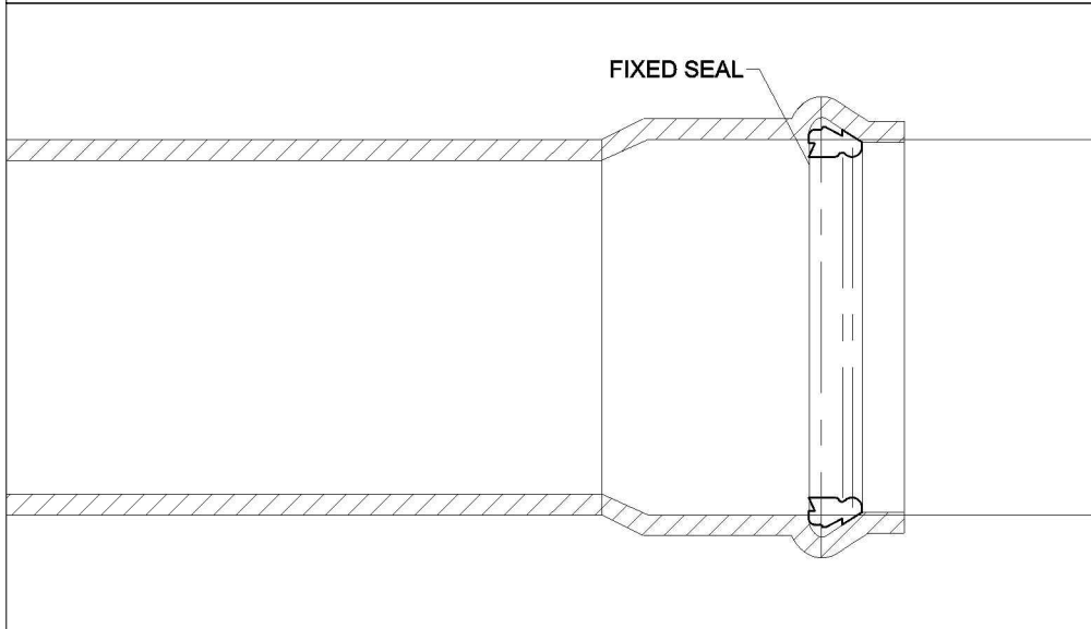
DETAIL A - RUBBER RING PIPE CONNECTION
